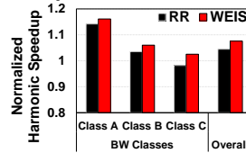
Figure 12: HS results for 100 workloads normalized with respect to FR-FCFS.
