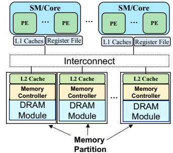
Fig. 1: Overview of our baseline GPU Architecture.
